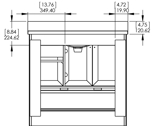
BACK VIEW
