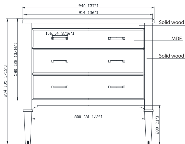
Front / Delantero
