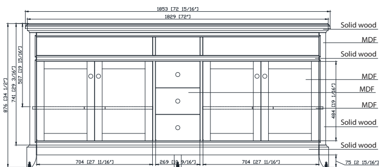
Front / Delantero
