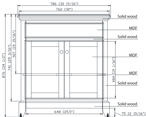
Front / Delantero
