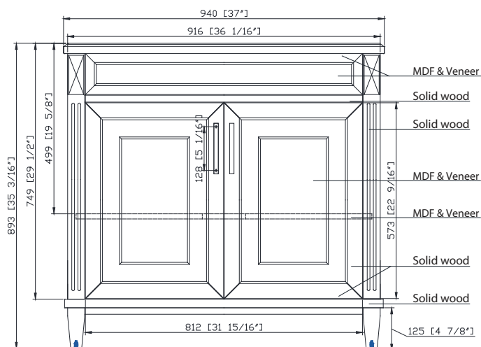
Front / Delantero
