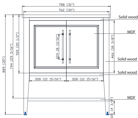
Front / Delantero
