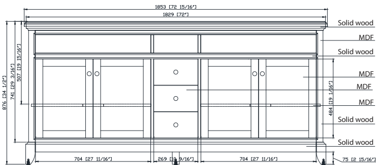
Front / Delantero
