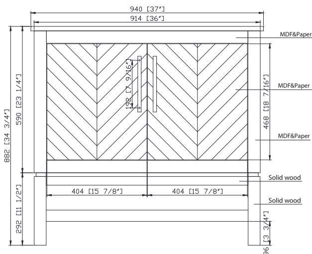
Front / Delantero
