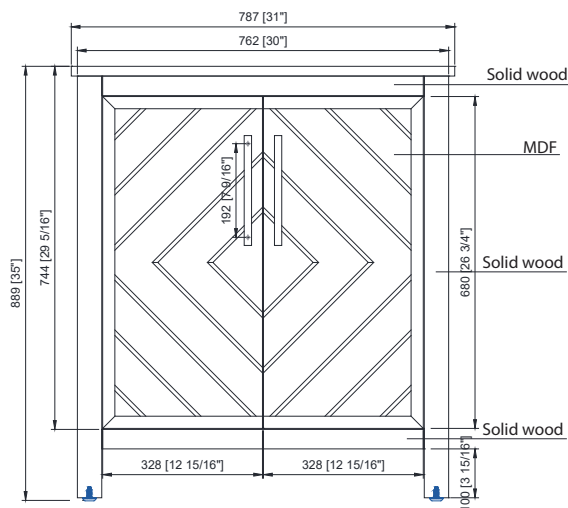
Front / Delantero
