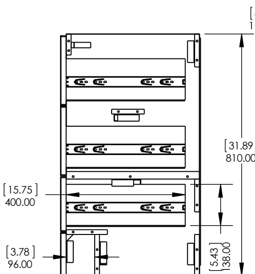
Side View / Vista Lateral
