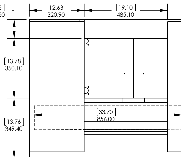
Back View / Vista Trasera
