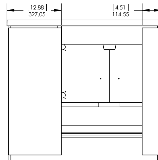
Back View / Vista Trasera
