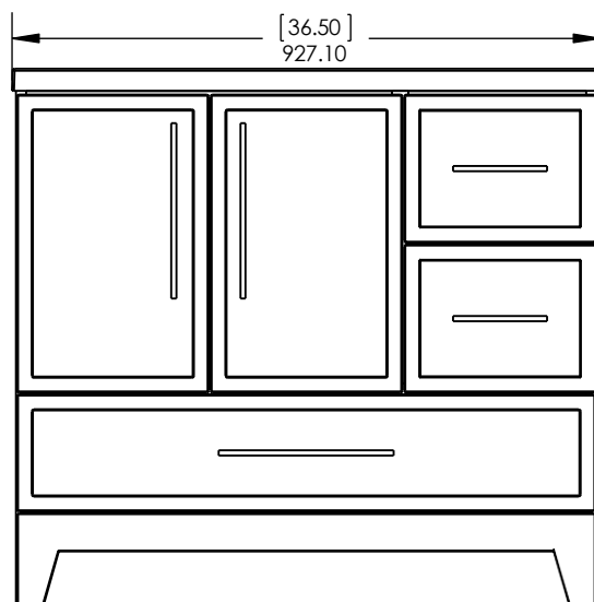
Front View / Vista Frontal
