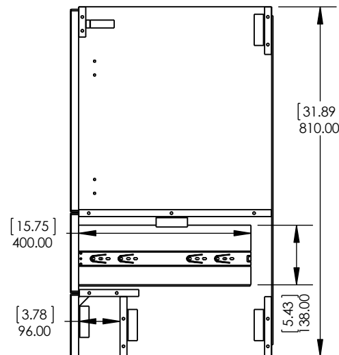
Side View / Vista Lateral
