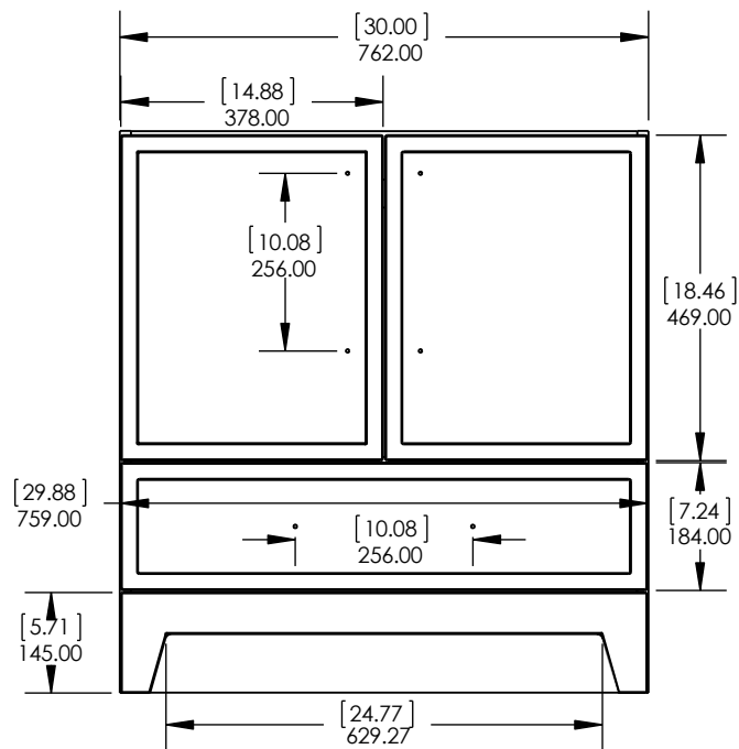
Front View / Vista Frontal
