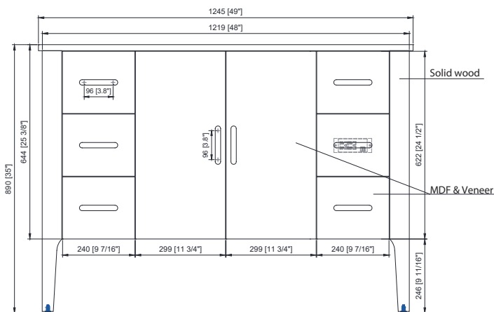
Front / Delantero
