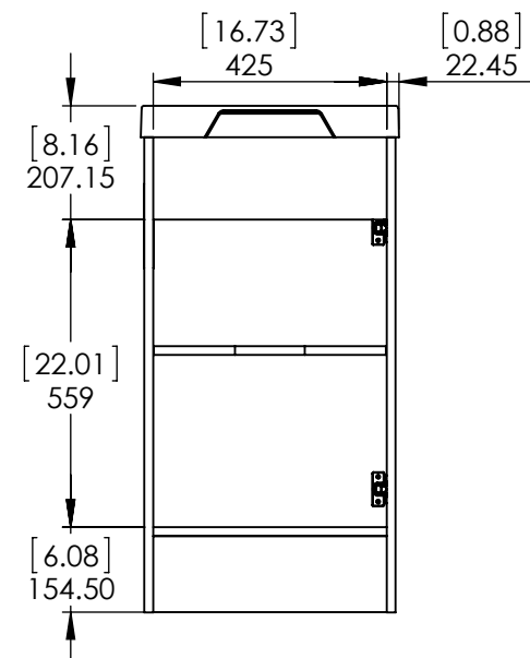
BACK VIEW
