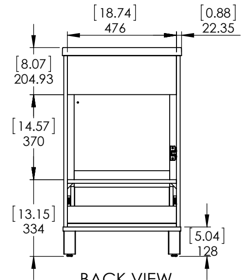
BACK VIEW
