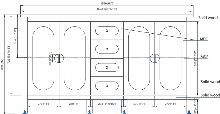
Front / Delantero
