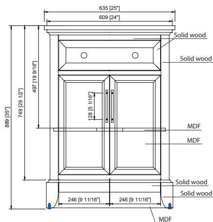
Front / Delantero
