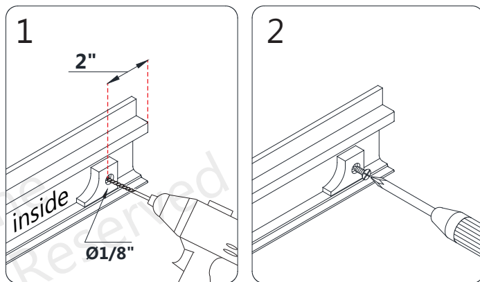
Fig 3 (Bottom Guide Rail shown)
